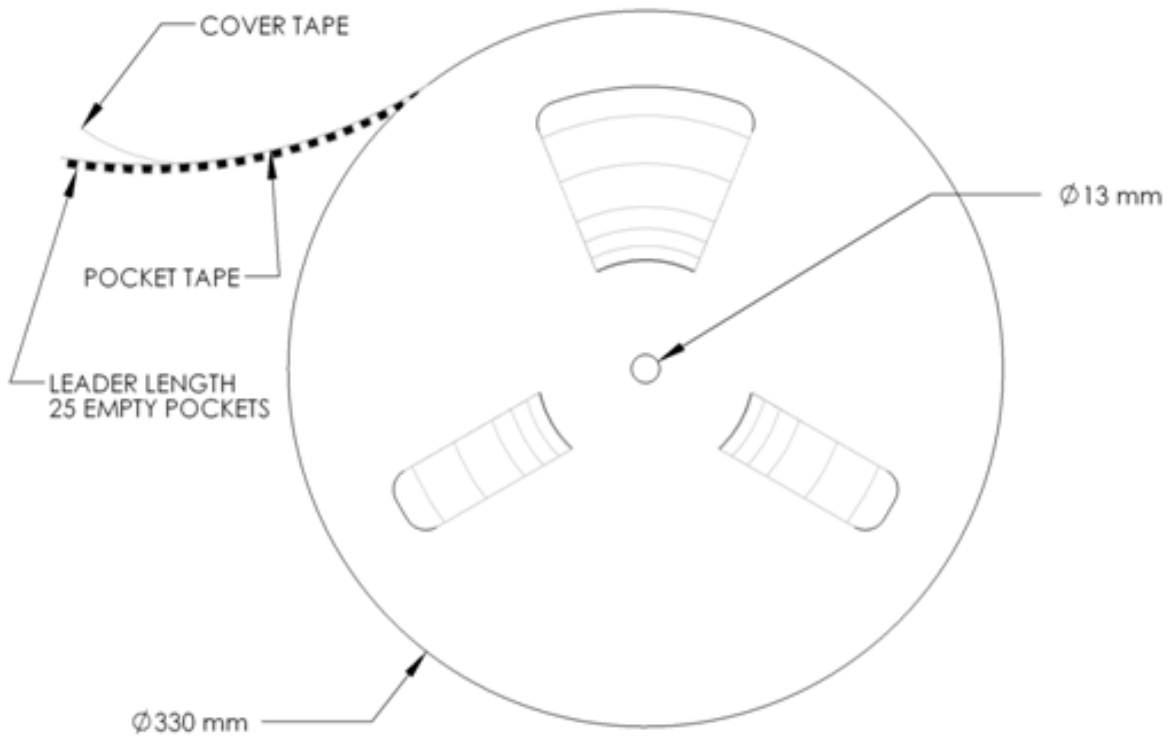
Figure 14: Emitter Reel specifications (mm).
