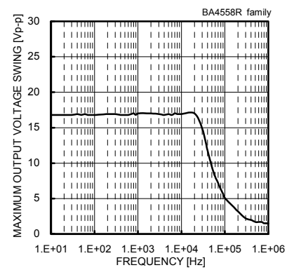
Maximum Output Voltage Swing - Frequency ( V_{CC}/V_{EE}=+15[V]/-15[V] , R_L=2[k\Omega] , T_a=25[°C] )
