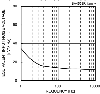
Equivalent Input Noise Voltage - Frequency ( V_{CC}/V_{EE}=+15[V]/-15[V] , R_s=100[\Omega] , T_a=25[°C] )
