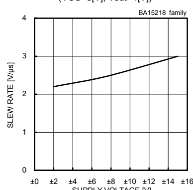
Fig. 216 Slew Rate - Supply Voltage (CL=100[pF], RL=2[kΩ], Ta=25[°C])
