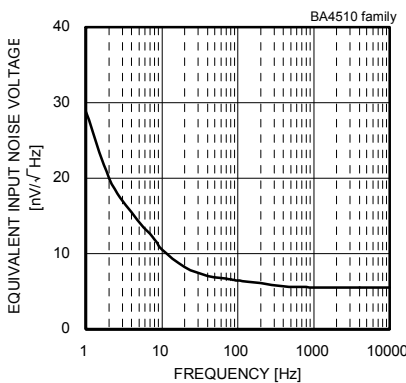
Fig. 286 Equivalent Input Noise Voltage - Frequency ( V_{CC}/V_{EE}=2.5[V]/-2.5[V] )
