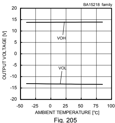
Maximum Output Voltage - Ambient Temperature (VCC/VEE=+15[V]/-15[V], RL=2[kΩ])
