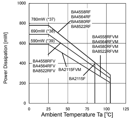
(c)BA4558R/BA4560R/BA4580R/BA8522R/BA2115 family
