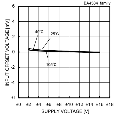
Fig. 141 Input Offset Voltage - Supply Voltage (Vcm=0[V], Vout=0[V])
