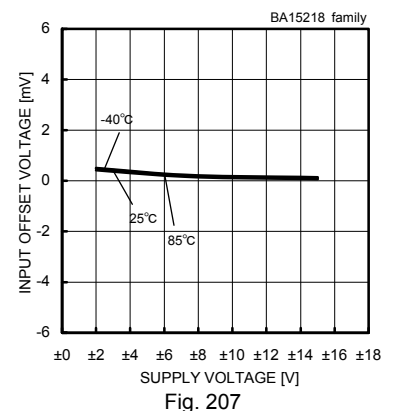
Input Offset Voltage - Supply Voltage (Vcm=0[V], Vout=0[V])
