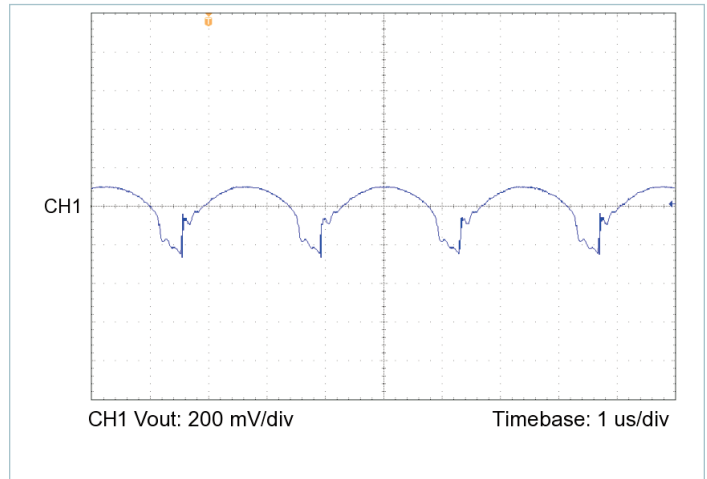
Figure 19 — Output voltage ripple, V_{IN} = 48\text{ V} , V_{OUT} = 5.0\text{ V} , C_{OUT\_EXT} = 1000\text{ }\mu\text{F} , R_{LOAD} = 0.156\text{ }\Omega
