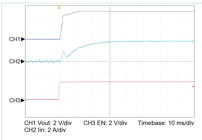
Figure 17 — Startup from EN, V_{IN} = 48\text{ V} , C_{OUT\_EXT} = 10000\text{ }\mu\text{F} , R_{LOAD} = 0.156\text{ }\Omega
