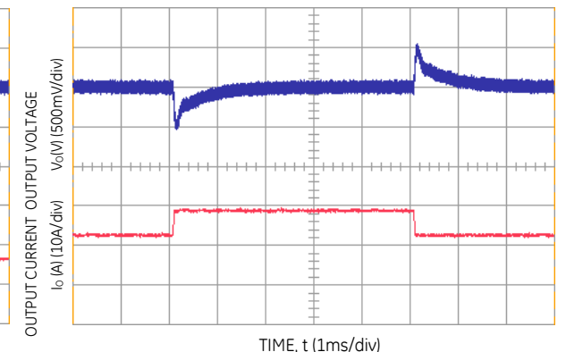
Figure 6. Transient Response to Dynamic Load Change from 50% to 75% to 50% of Full Load at Room Temperature and 48 Vdc Input; 0.1A/µs ; C_{o,ext} = 470\mu F .
