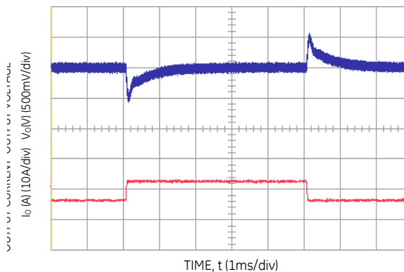
Figure 3. Transient Response to Dynamic Load Change from 25% to 50% to 25% of Full Load at Room Temperature and 48 Vdc Input; 0.1A/µs ; C_{o,ext} = 470\mu F .
