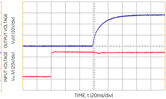
Figure 5. Typical Start-Up Using from V_{IN} , positive logic version shown; C_{o,ext} = 470\mu F .
