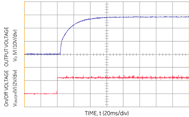
Figure 4. Typical Start-Up Using Remote On/Off, R1=30k\Omega ; C_{o,ext} = 470\mu F .
