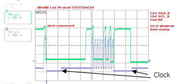
Figure 1. Example waveforms showing clock stretch
