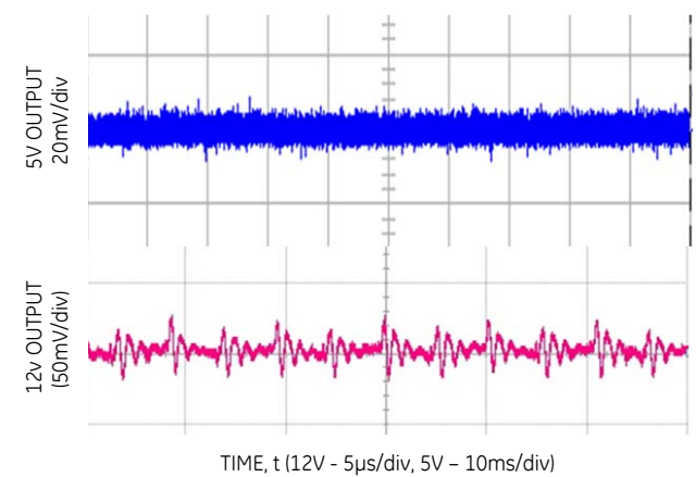
Figure 5. 12V output ripple and noise (Vin: -48V DC , full load).
