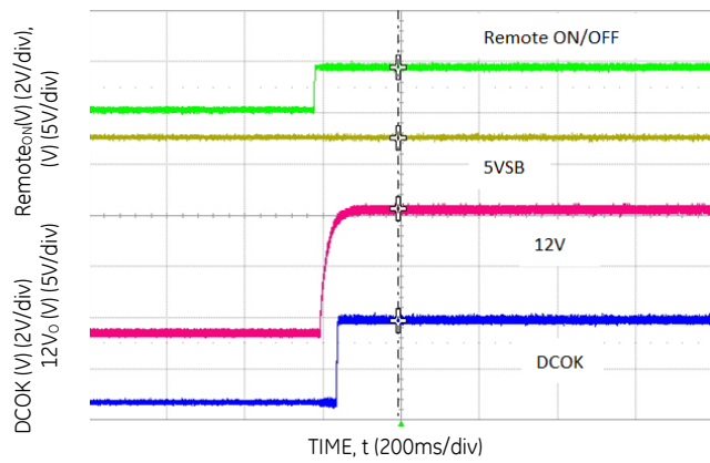
Figure 3. Start-up Using Remote On/OFF (Vin: -48V DC , full load)
