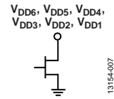
Figure 7. V_{DD6} to V_{DD1} Interface
