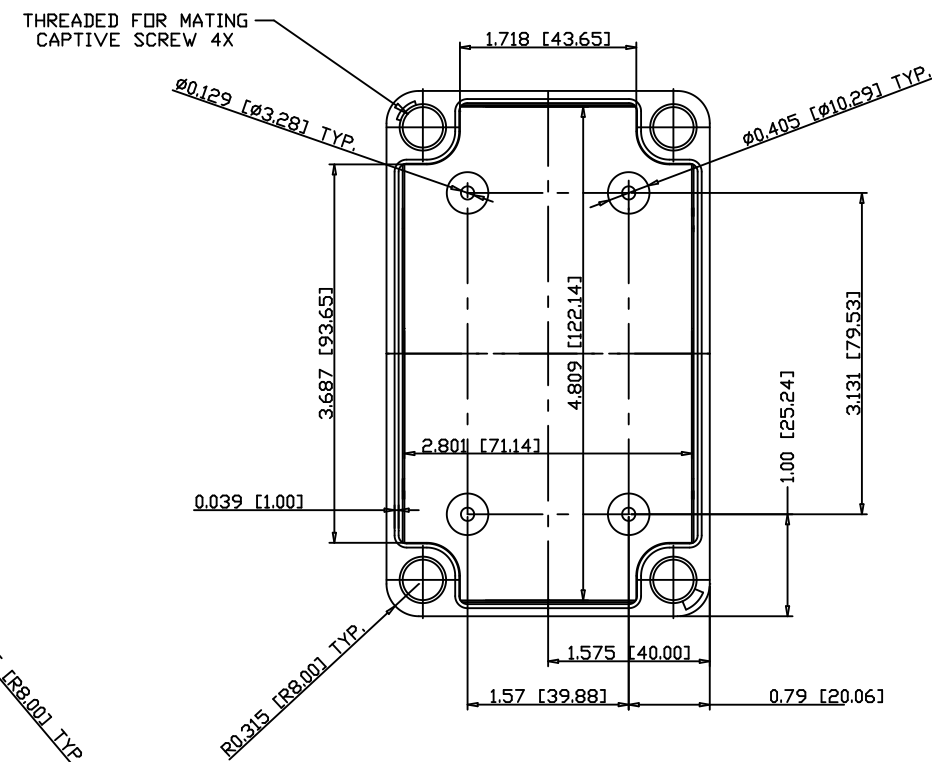
TOP VIEW WITH COVER REMOVED
