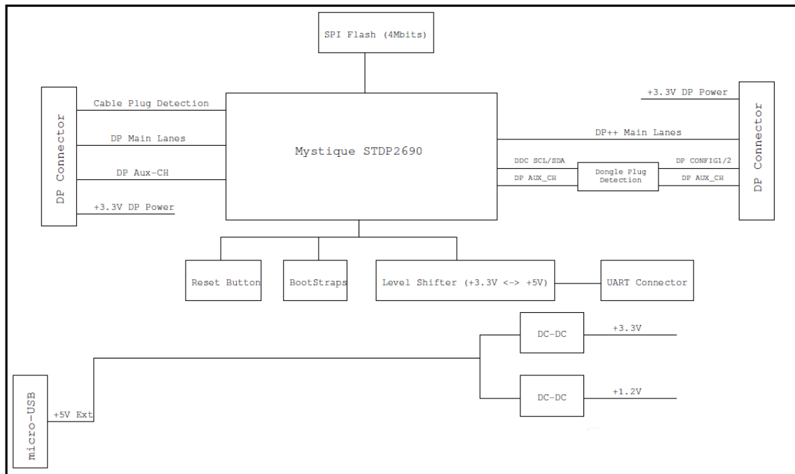
Figure 2. Connection diagram
