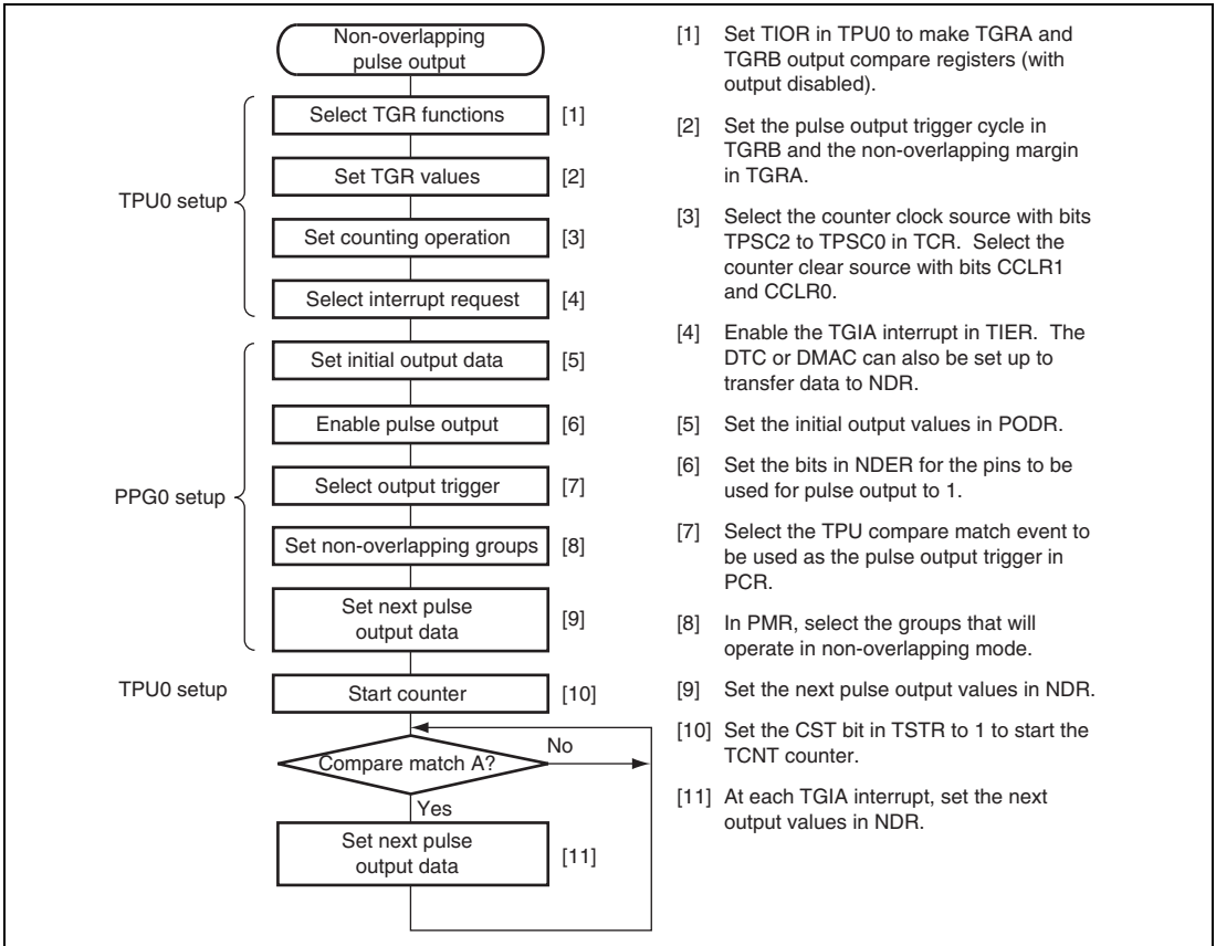
Figure 14.10 Setup Procedure for Non-Overlapping Pulse Output (PPG0)
