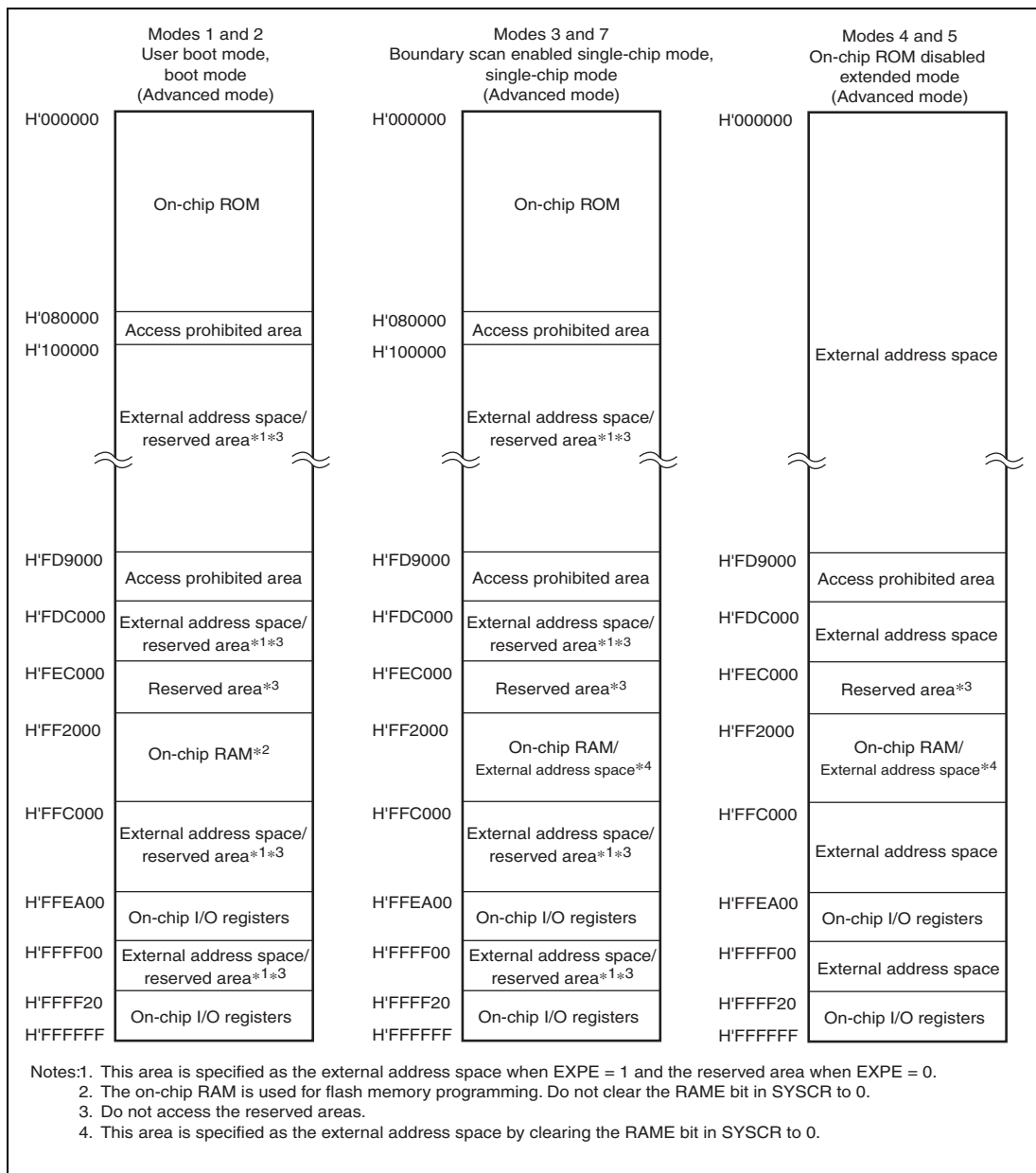
Figure 3.2 Address Map in Each Operating Mode of H8SX/1634 and H8SX/1634L (1)
