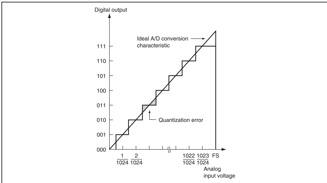
Figure 19.9 A/D Conversion Accuracy Definitions
