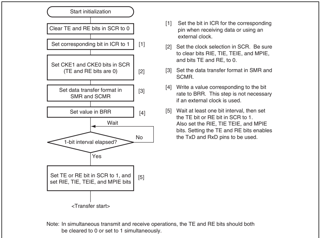
Figure 17.18 Sample SCI Initialization Flowchart
