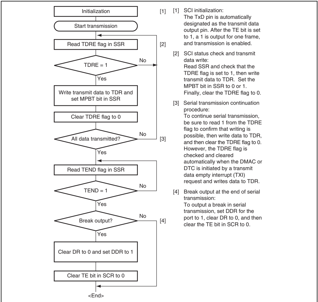
Figure 17.14 Sample Multiprocessor Serial Transmission Flowchart
