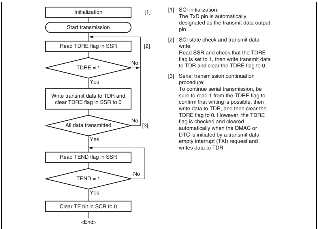
Figure 17.20 Sample Serial Transmission Flowchart
