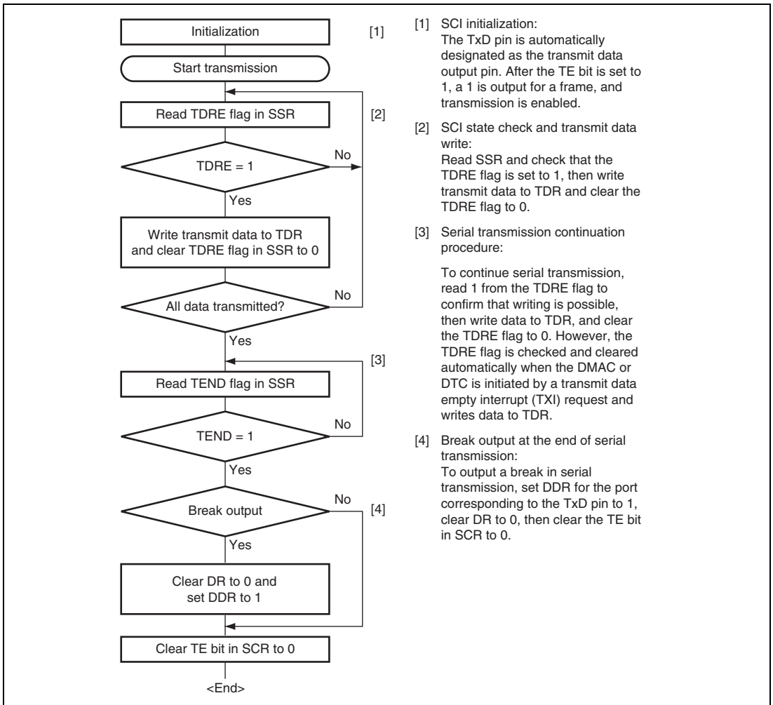
Figure 17.10 Example of Serial Transmission Flowchart
