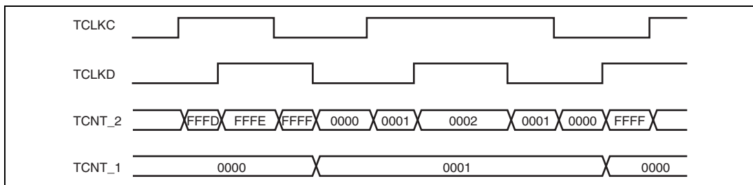
Figure 13.20 Example of Cascaded Operation (2)
