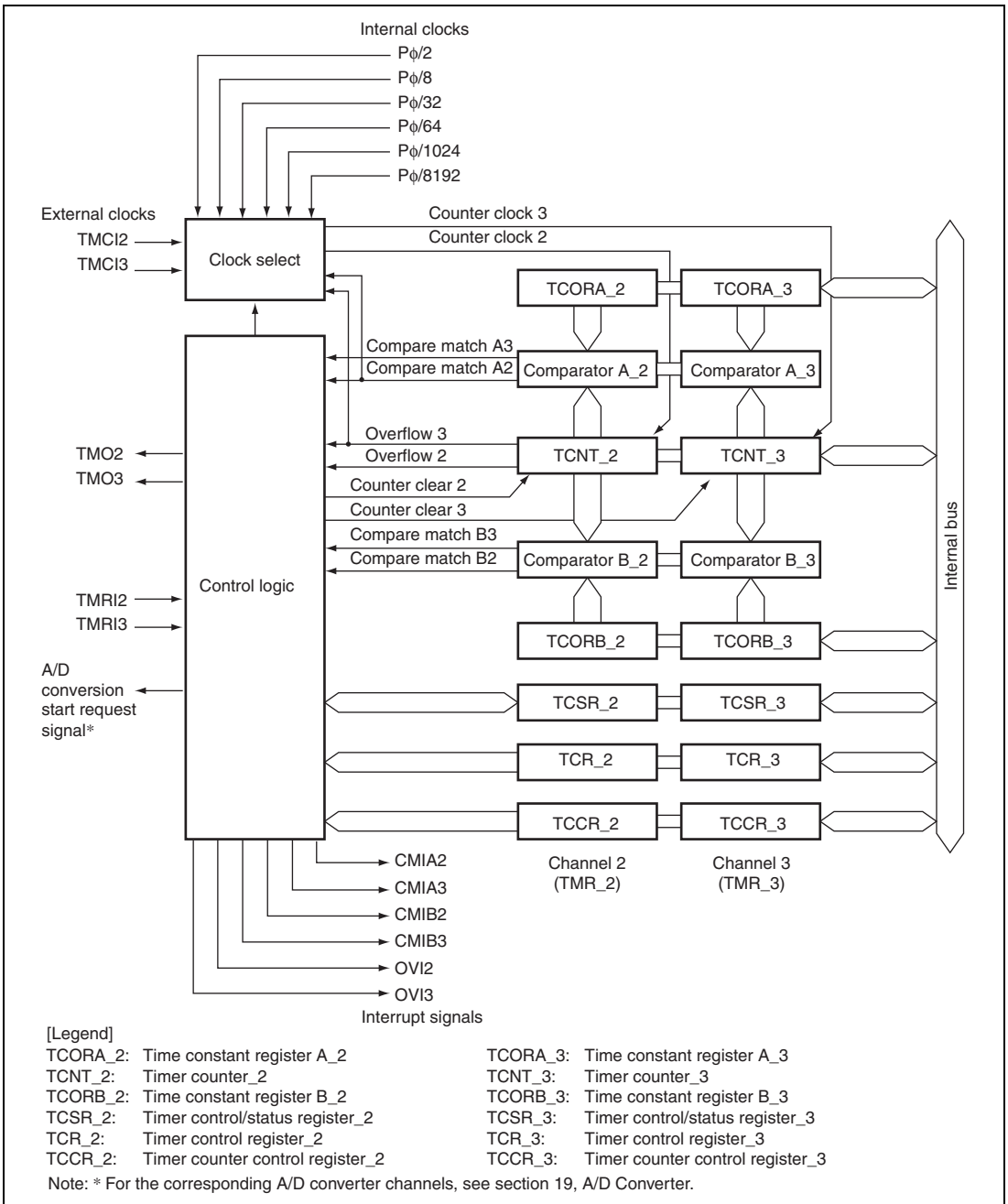
Figure 15.2 Block Diagram of 8-Bit Timer Module (Unit 1)
