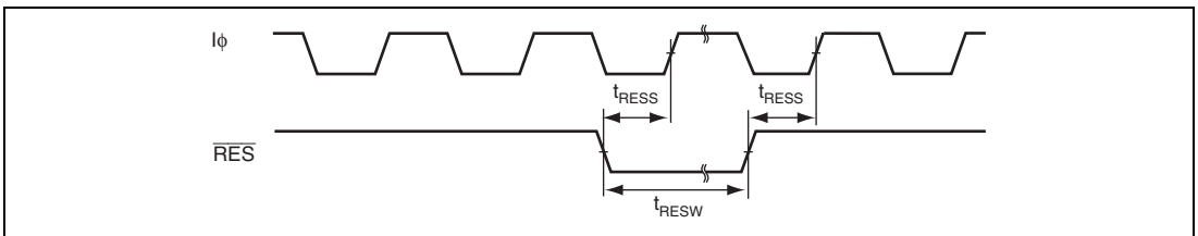
Figure 27.6 Reset Input Timing
