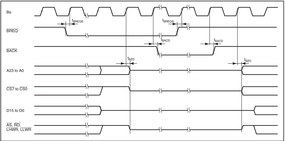
Figure 27.19 External Bus Release Timing
