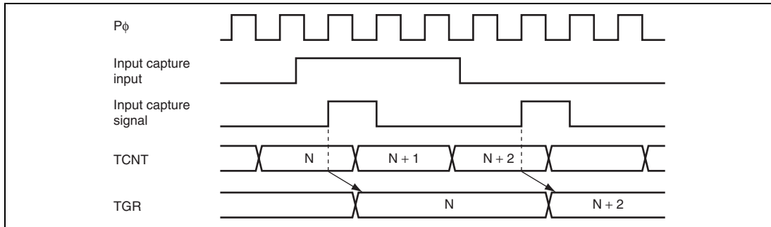
Figure 13.34 Input Capture Input Signal Timing
