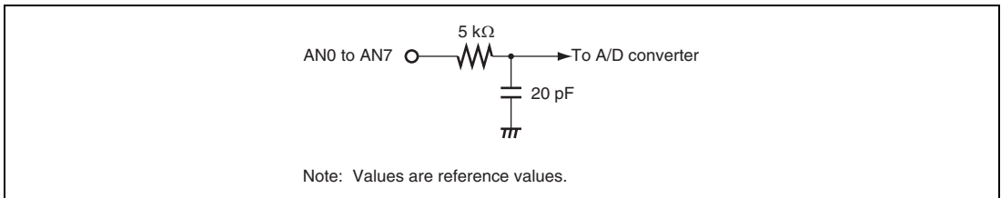
Figure 19.14 Analog Input Pin Equivalent Circuit
