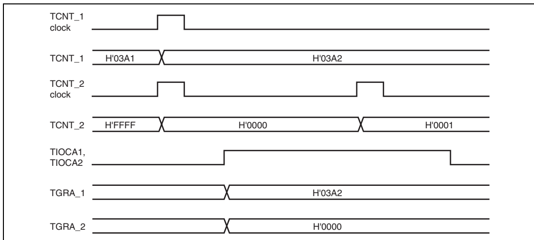
Figure 13.19 Example of Cascaded Operation (1)
