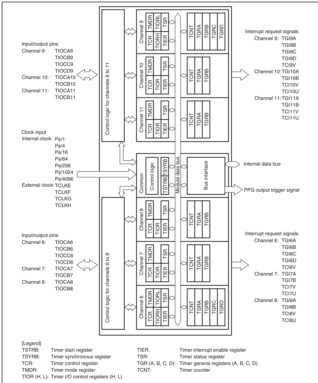
Figure 13.2 Block Diagram of TPU (Unit 1)
