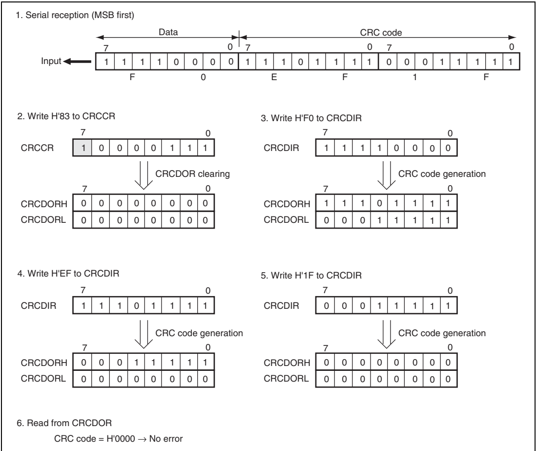
Figure 17.47 MSB-First Data Reception
