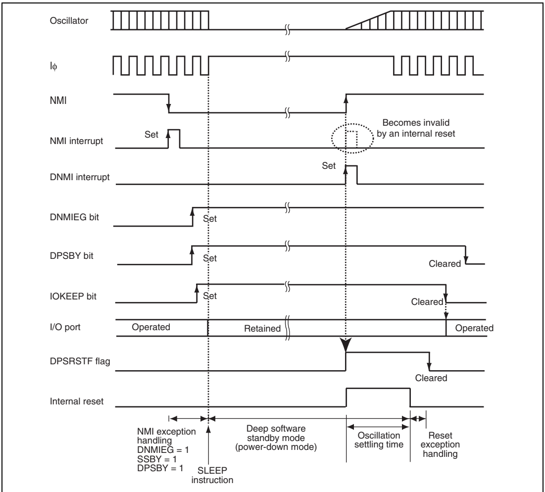
Figure 25.4 Deep Software Standby Mode Application Example (IOKEEP = 1)
