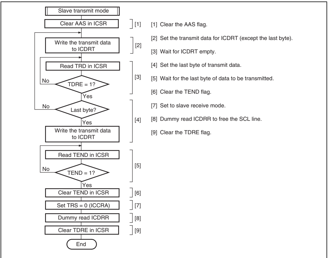
Figure 18.16 Sample Flowchart for Slave Transmit Mode
