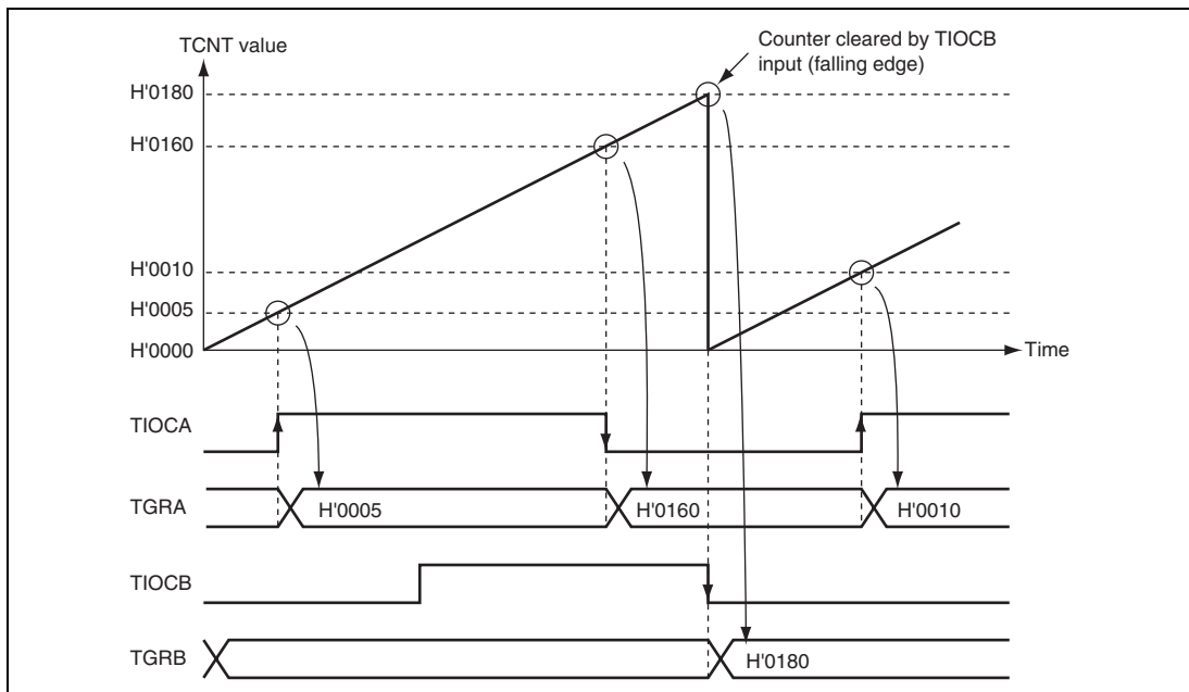
Figure 13.10 Example of Input Capture Operation
