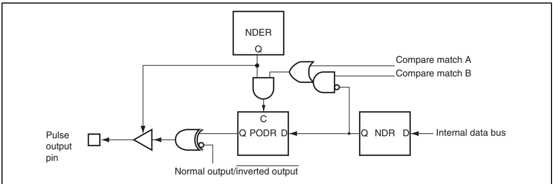
Figure 14.8 Non-Overlapping Pulse Output
