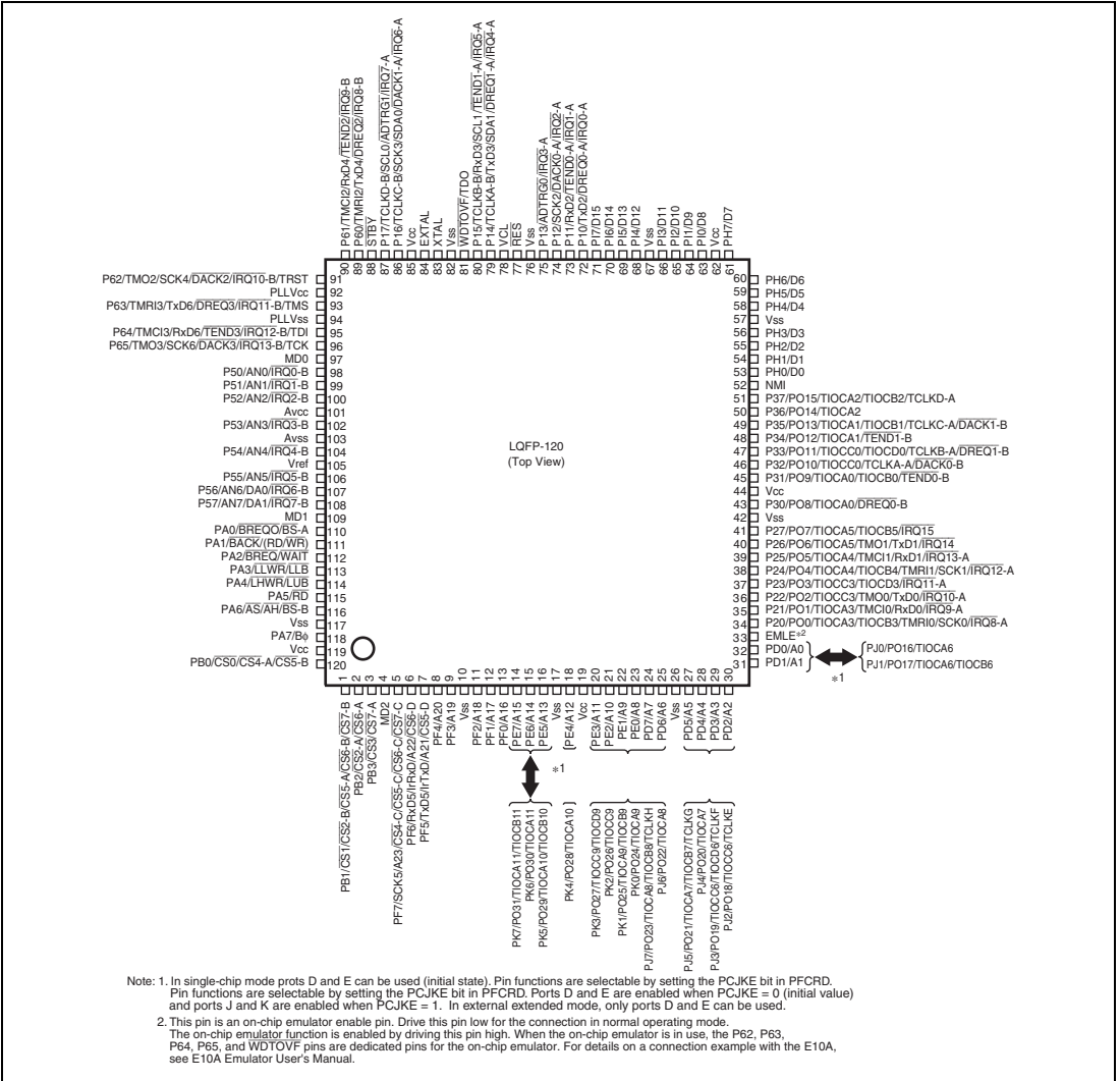
Figure 1.3 Pin Assignments
