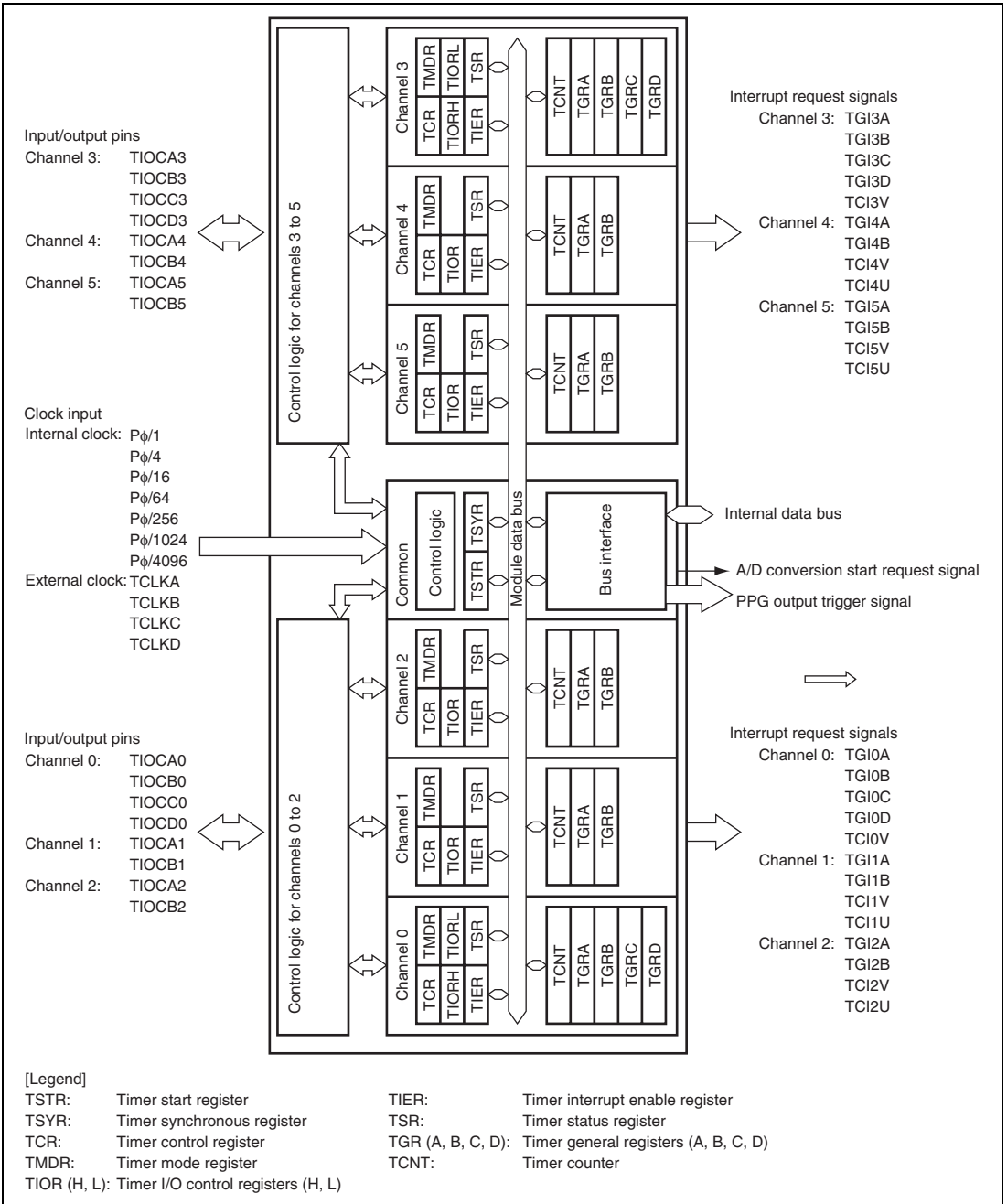
Figure 13.1 Block Diagram of TPU (Unit 0)
