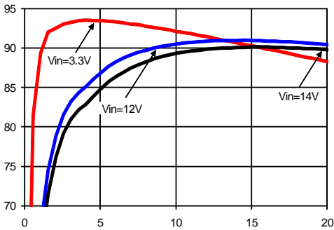
Figure 1. Vo=0.6V
