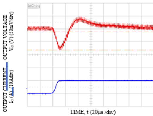
Transient Response to Dynamic Load Change from 50% to 100% at 12Vin, C_{out} = 5 \times 47\mu F + 1 \times 330\mu F , C_{Tune} = 2200pF & R_{Tune} = 220 \text{ ohms} , V_o = 3.3V
