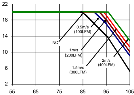
Figure 7. V_o=0.6V
