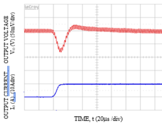
Transient Response to Dynamic Load Change from 50% to 100% at 12Vin, C_{out} = 8 \times 47\mu F , C_{Tune} = 1500pF & R_{Tune} = 220 \text{ ohms} , V_o = 5.0V
