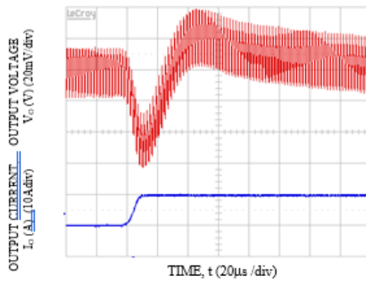
Transient Response to Dynamic Load Change from 50% to 100% at 12Vin, C_{out} = 2 \times 47\mu F + 2 \times 330\mu F , C_{Tune} = 3300pF & R_{Tune} = 220 \text{ ohms} , V_o = 2.5V
