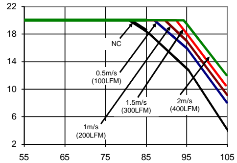
Figure 8. V_o=1.2V
