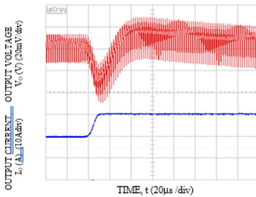
Transient Response to Dynamic Load Change from 50% to 100% at 12Vin, C_{out} = 2 \times 47\mu F + 3 \times 330\mu F , C_{Tune} = 5600pF & R_{Tune} = 220 \text{ ohms} , V_o = 1.8V
