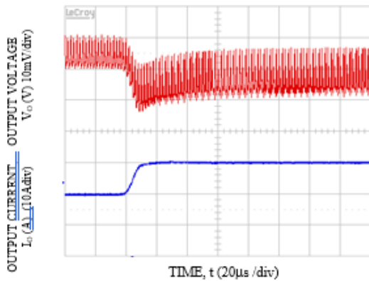
Transient Response to Dynamic Load Change from 50% to 100% at 12Vin, C_{out} = 1 \times 47\mu F + 11 \times 330\mu F , C_{Tune} = 47nF , R_{Tune} = 178 \text{ ohms} , V_o = 0.6V
