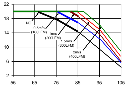
Figure 12. V_o=5.0V
