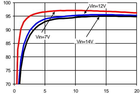
Figure 4. Vo=2.5V
