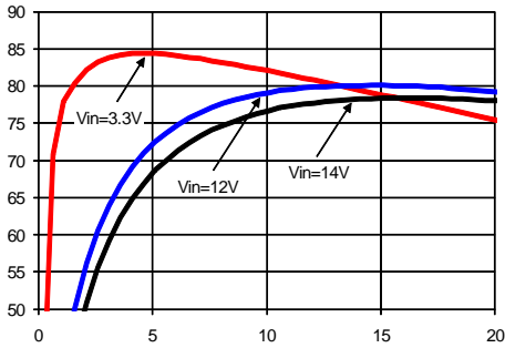
Figure 1. Vo=0.6V
