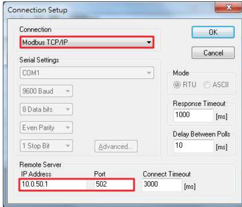
Figure 2.27 Modbus Poll Connection Setup
