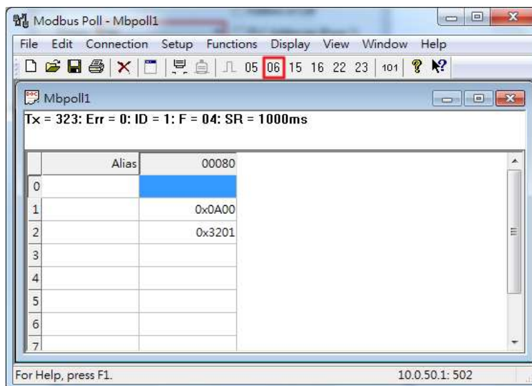
Figure 2.37 Click on Function 06 in the Modbus Poll
