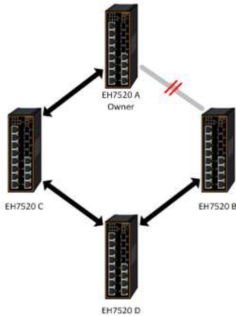
Figure 2.129 Example of Ring Topology for ERPS Setup
