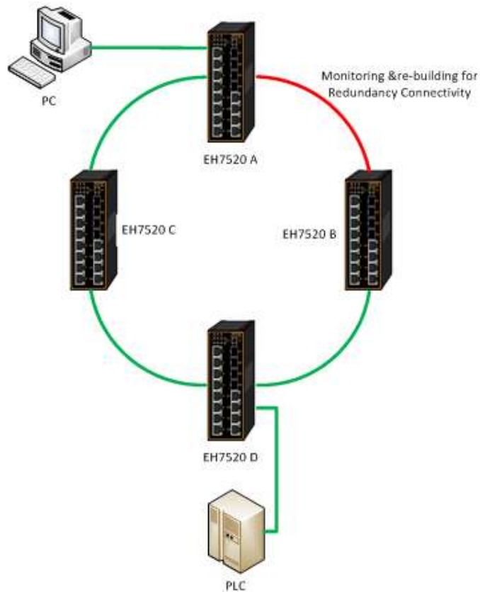
Figure 2.134 iA-Ring Example Topology
