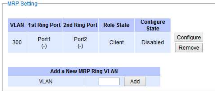
Figure 2.149 Example of PROFINET's MRP VLAN Entry
