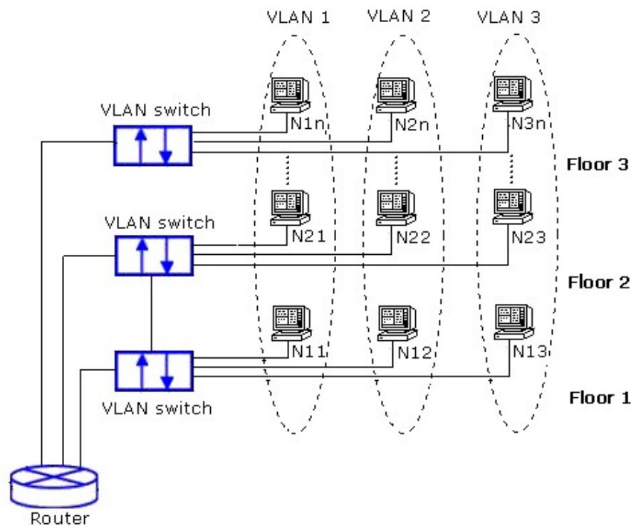
Figure 2.101 Example of VLAN Configuration
