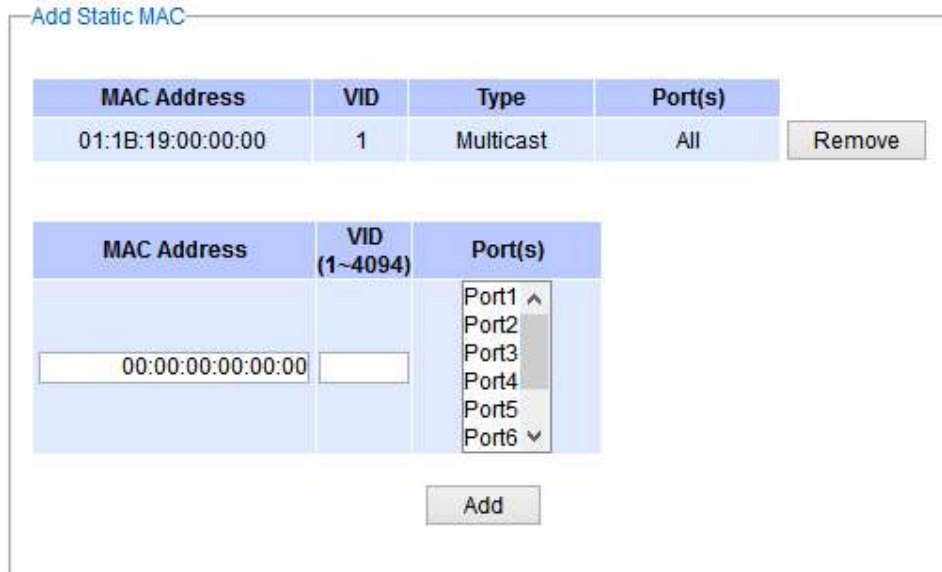
Figure 2.67 Add Static MAC Webpage
