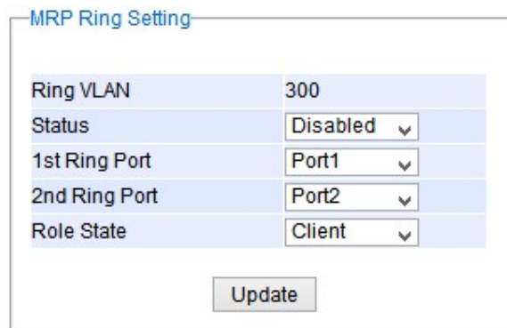
Figure 2.150 MRP Ring Setting Webpage
