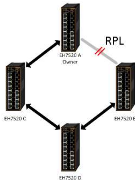
Figure 2.125 An Example of Ring Topology
