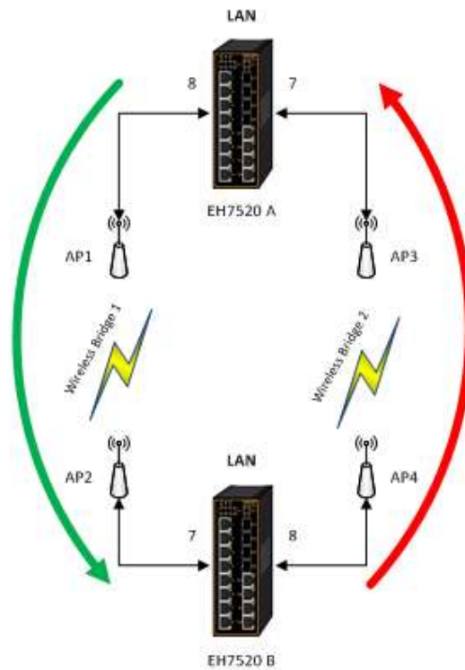
Figure 2.137 Example 1 of Two Wireless Bridge U-ring
