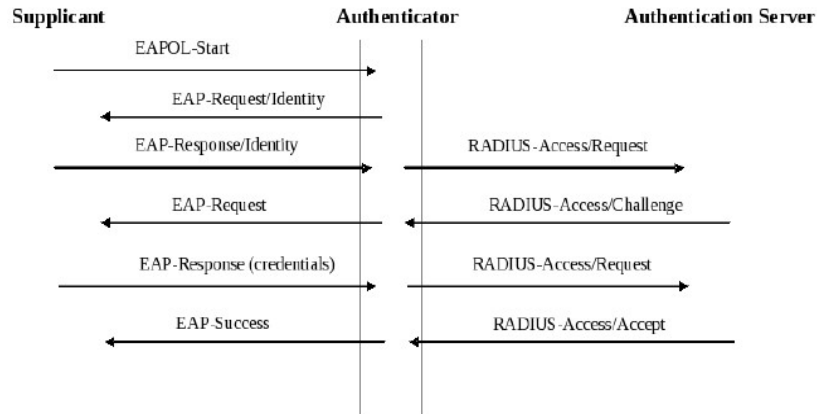
Figure 2.119 RADIUS Authentication Sequence
