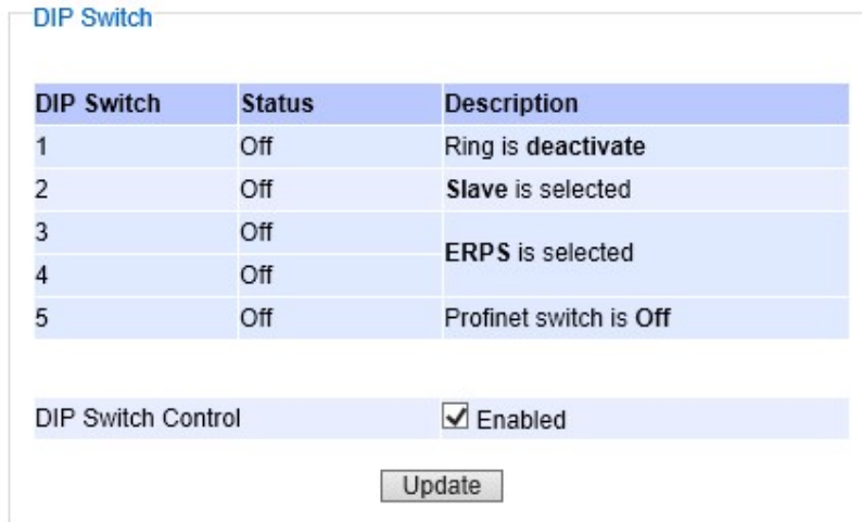
Figure 2.45 DIP Switch Status Webpage
