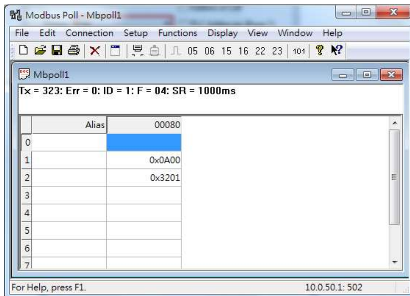
Figure 2.34 Modbus Memory Address 81 and 82 are the location of EHG7508's IP Address
