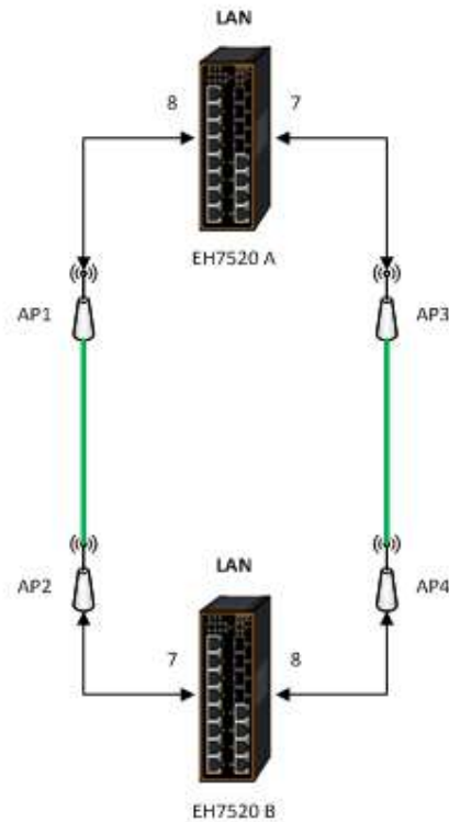
Figure 2.138 Example 2 of Two Wired Bridge U-ring
