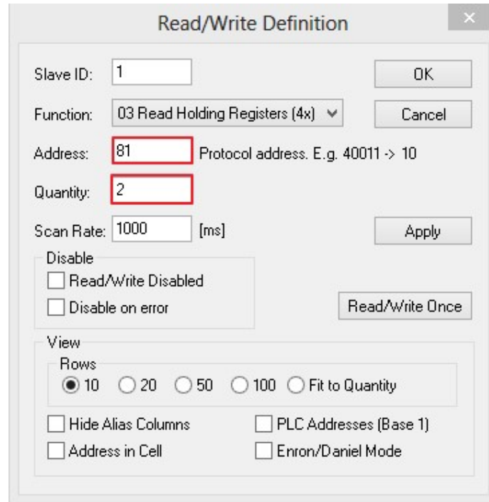
Figure 2.33 Setup Starting Address and Quantity in Modbus Poll
