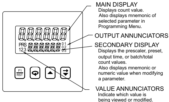
Figure 10 , Front Panel
