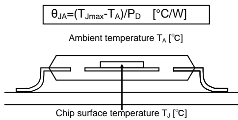
Figure 17. Thermal resistance
