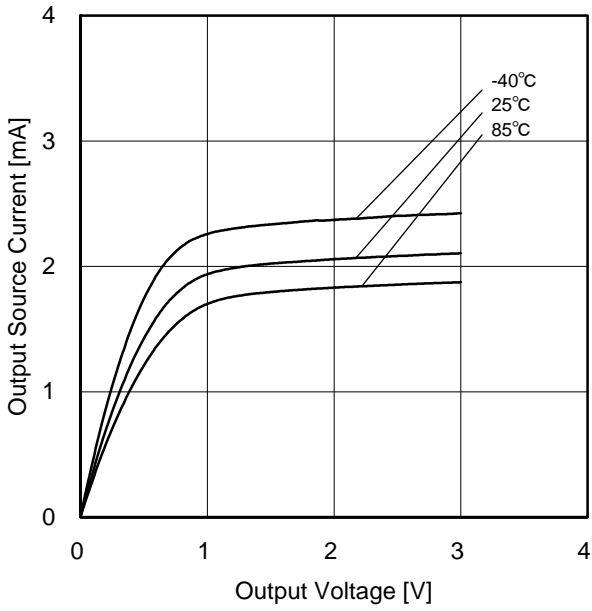
Figure 9. Output "L" Current vs Output Voltage ( V_{DD}=3V / V_{SS}=0V )
