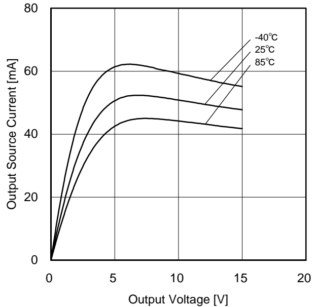
Figure 12. Output "L" Current vs Output Voltage ( V_{DD}=15V / V_{SS}=0V )
