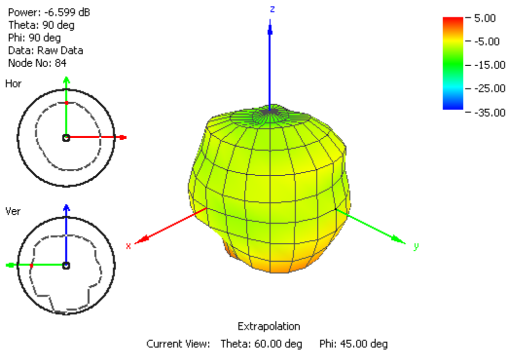
Figure15. Radiation Pattern at 1710 MHz of G30 Antenna in Free Space
