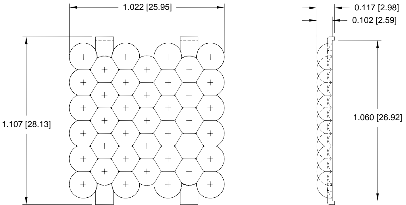
Figure 2 – Mechanical Dimensions
