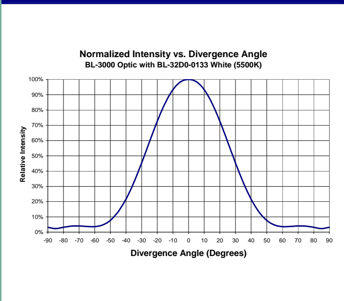
Figure 1 – Total Beam Divergence
