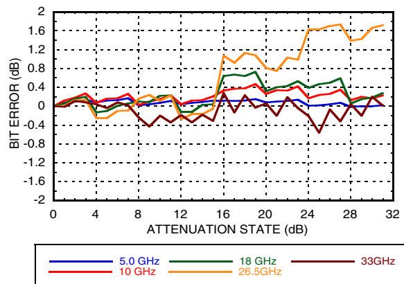
Bit Error vs. Attenuation State
