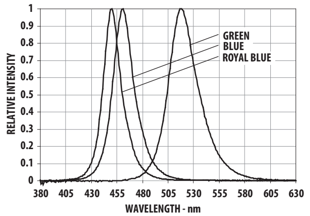
Figure 13. Relative Intensity vs. Wavelength for Blue, Royal Blue and Green
