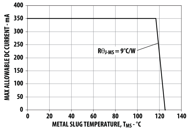
Figure 11. Maximum Forward Current vs. Ambient Slug Temperature. Derated based on T_{JMAX} = 125^{\circ}C , R_{\theta j-ms} = 9^{\circ}C/W
