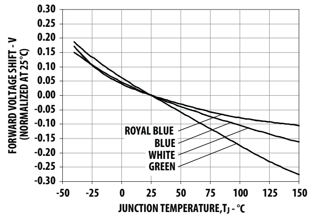
Figure 21. Forward Voltage Shift vs. Junction Temperature
