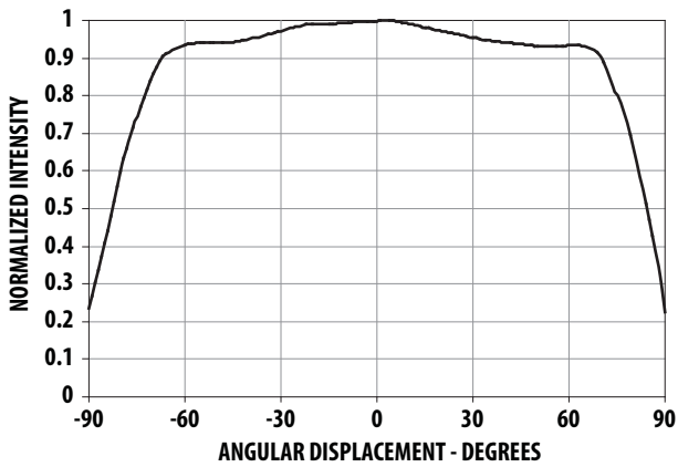
Figure 16. Radiation Pattern for Blue, Royal Blue and Green
