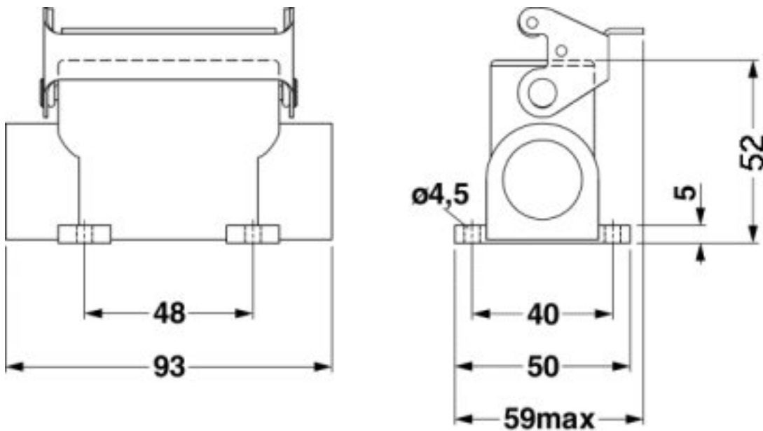
Dimensioned drawing
