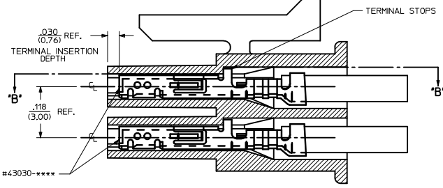
SECTION 'A'-A' WITH TERMINAL (SCALE 10:1)
