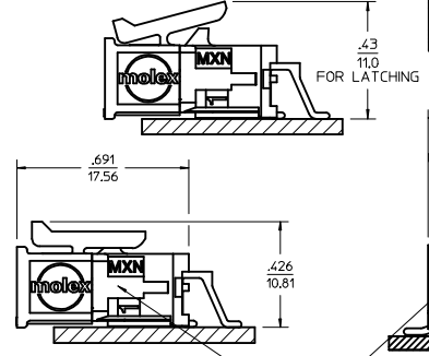
MATED MICRO-FIT CONNECTOR
