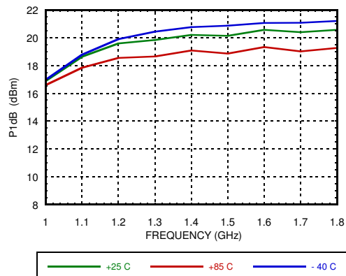
Output P1dB vs. Temperature [1]
