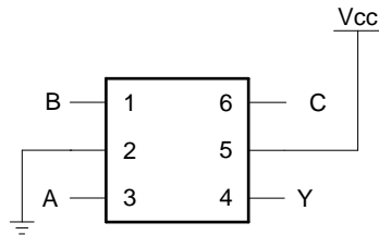
Configuration 1 2 to 1 Data Selector When C is = L, Y = \bar{B} ; When C is H, Y = \bar{A}
