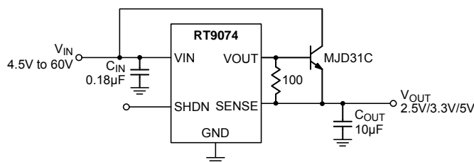
Figure 3. RT9074-25/33/50 External Transistor Application
