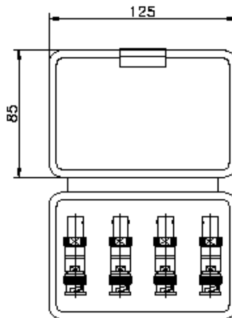
120086 Attenuator Kit Case Dimensions (mm)
