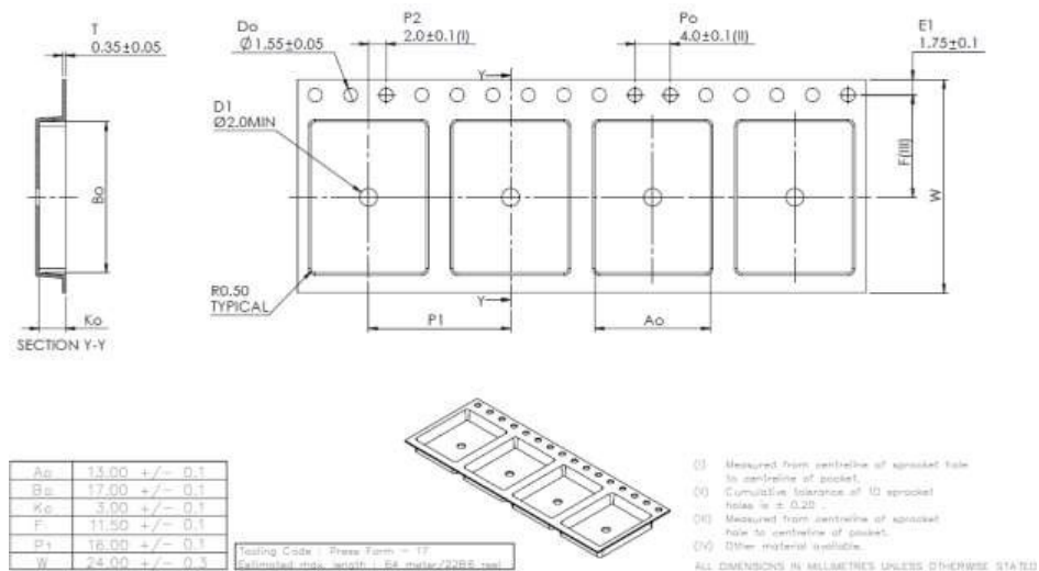
Figure 15-3 Tape and Reel – Tape detail
