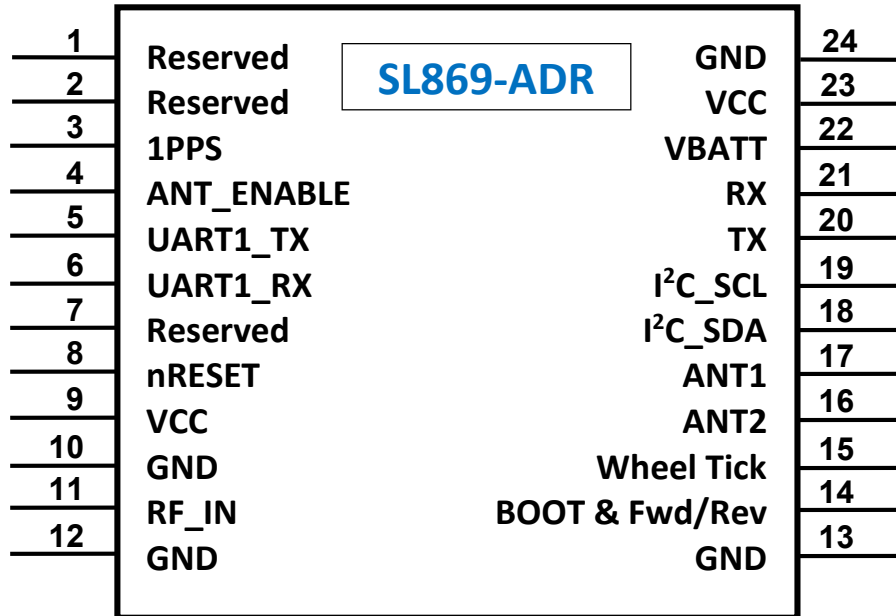
Figure 10-1 SL869-ADR Pin-out Diagram
