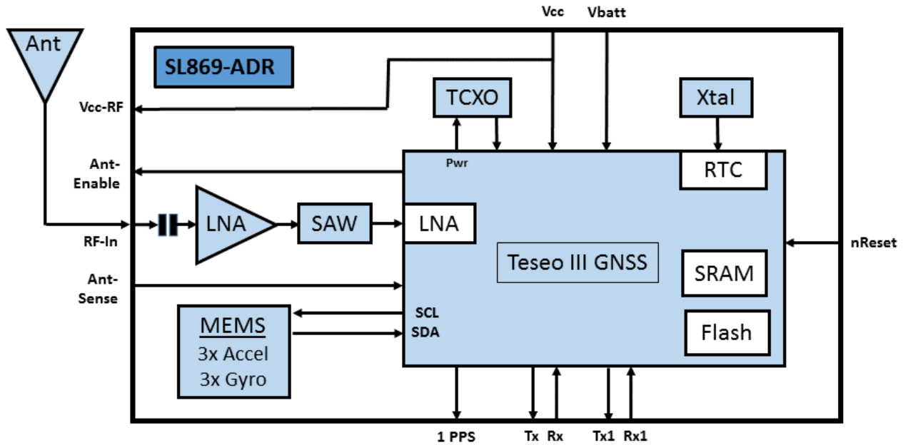
Figure 2-1 SL869-ADR Block Diagram
