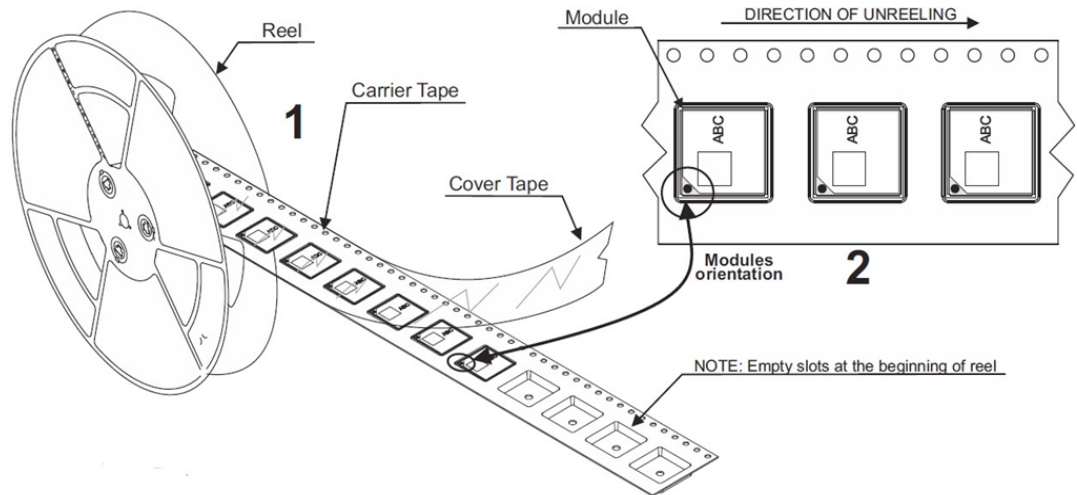
Figure 15-2 Tape and Reel Packaging
