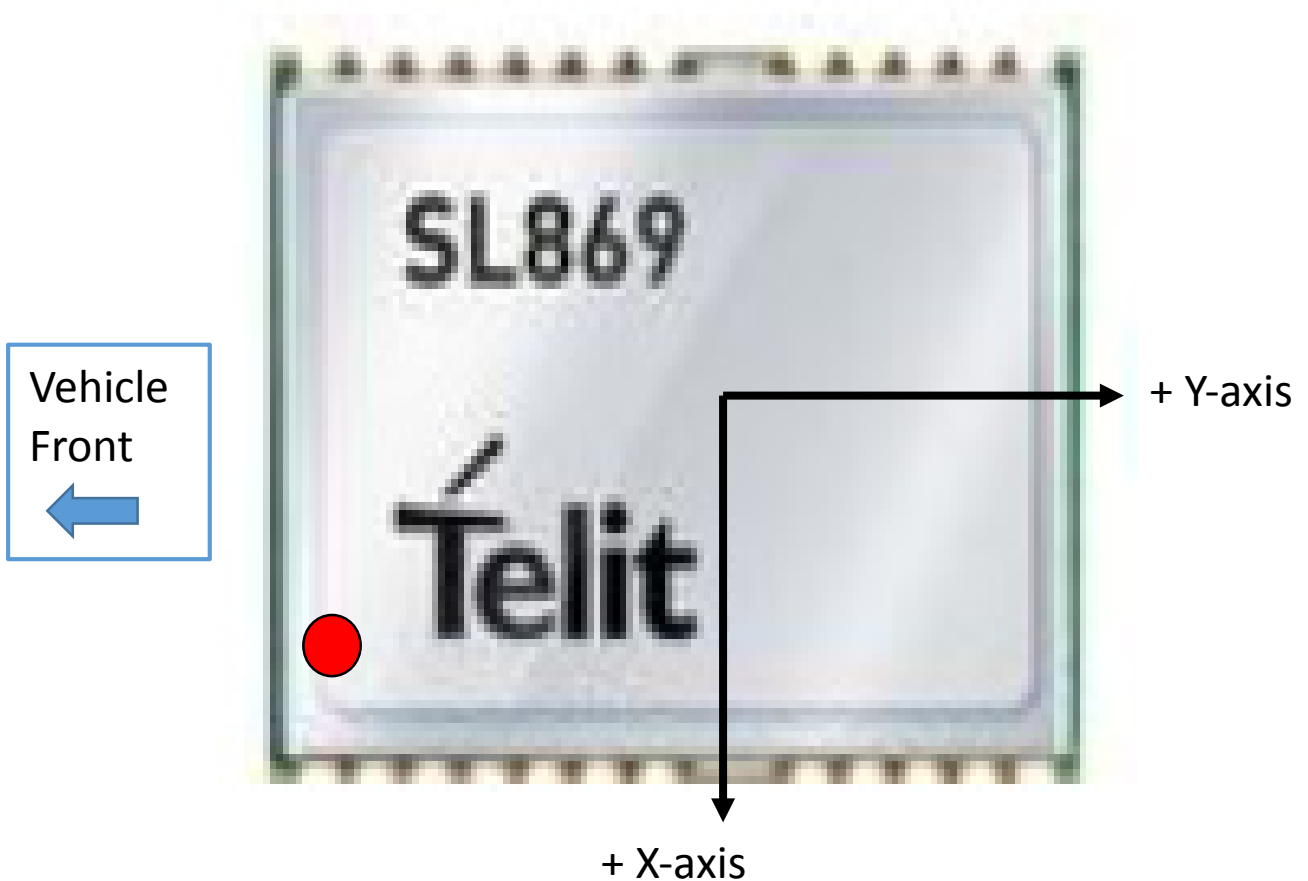
Figure 6-1 Module Orientation
