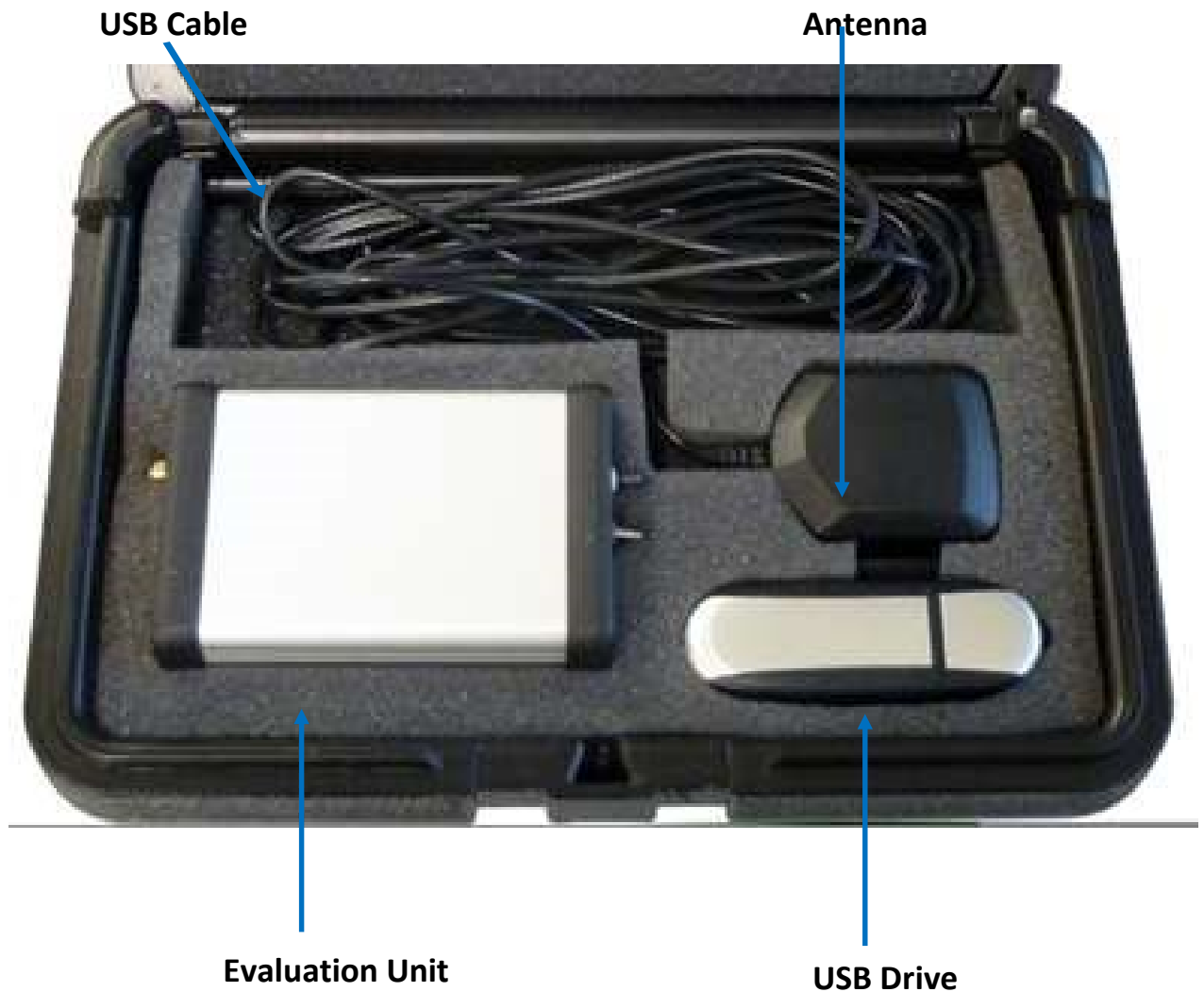
Figure 3-1 SL869-ADR EVK
