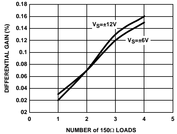
FIGURE 16. DIFFERENTIAL GAIN
