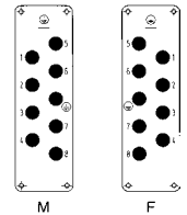
Contact arrangement (view from termination side)
