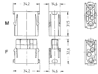
Contact arrangement (view from termination side)
