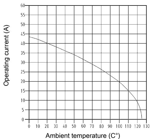
Wire cross section 4 mm 2
