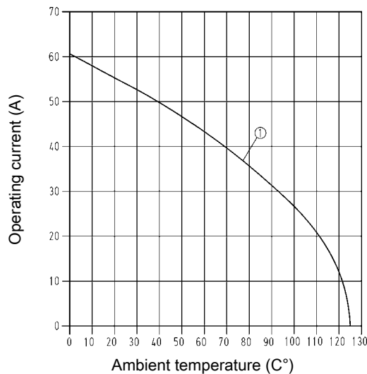
Energy supply Wire cross section 10 mm 2
